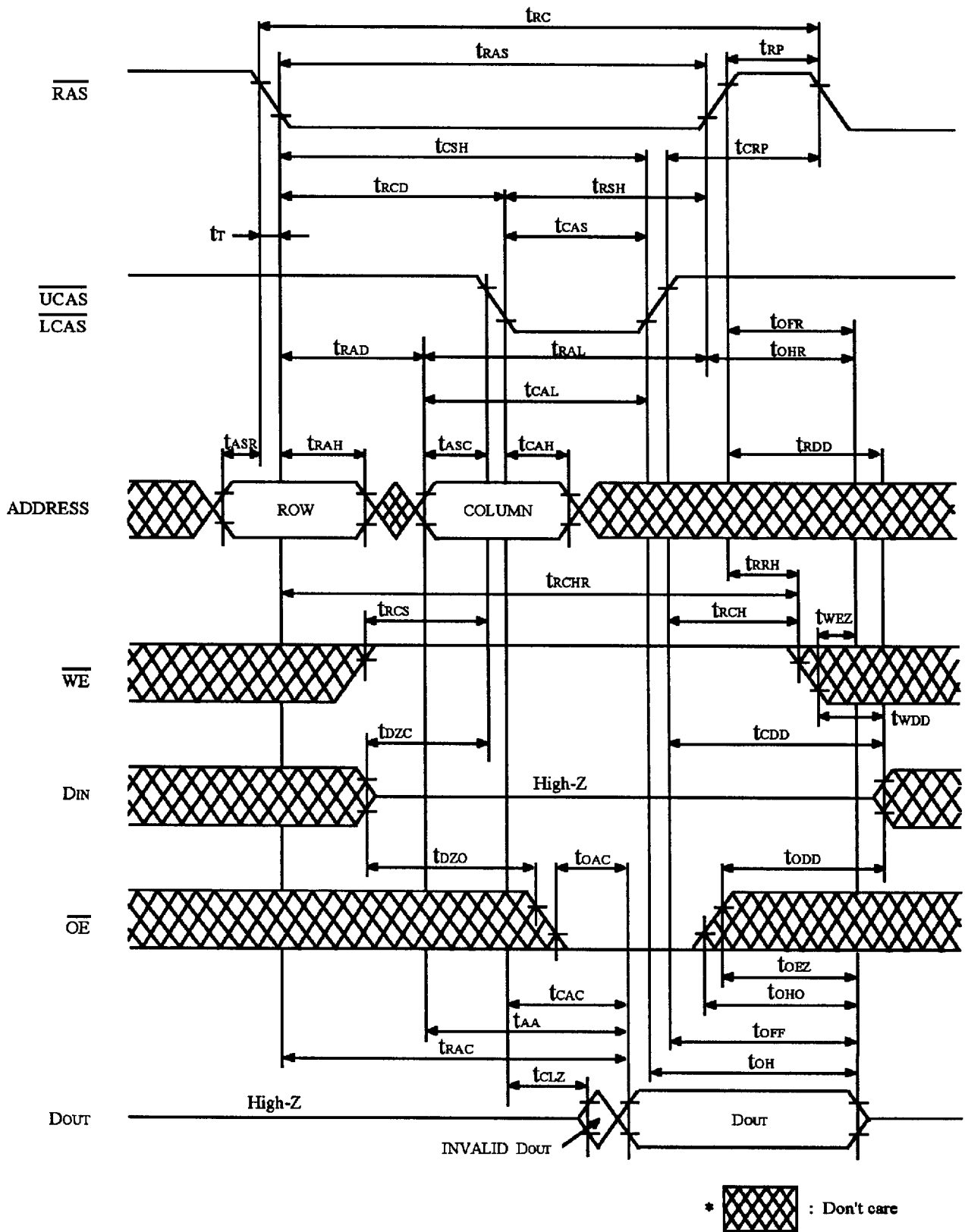
FIGURE 1. READ CYCLE
