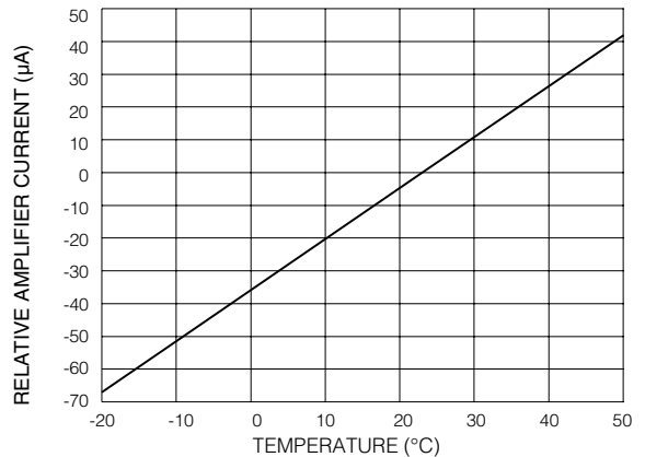
Fig. 9 Amplifier Current vs Temperature
