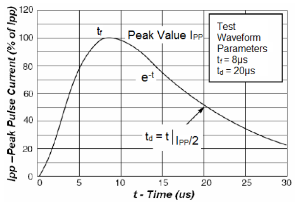
Figure 2. Pulse Waveform
