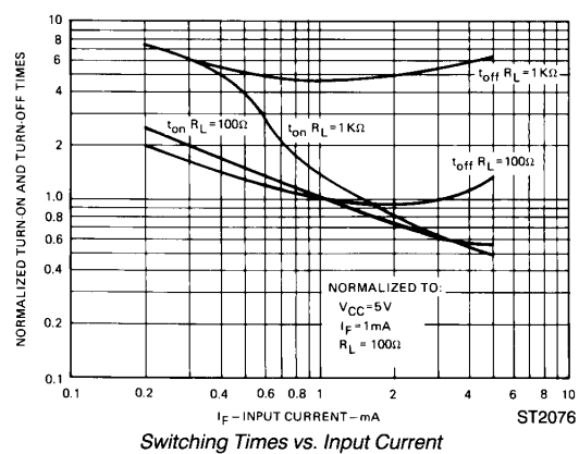
Switching Times vs. Input Current
