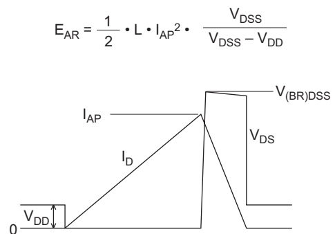
Avalanche Waveform
