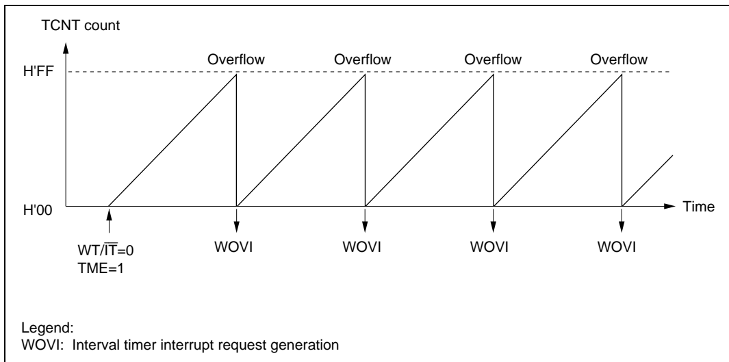
Figure 15.5 Interval Timer Operation
