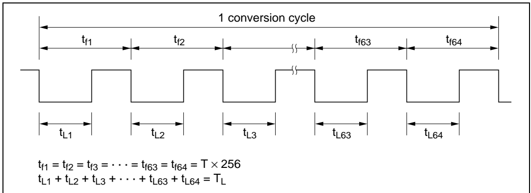
Figure 14.4 (2) Output Waveform
