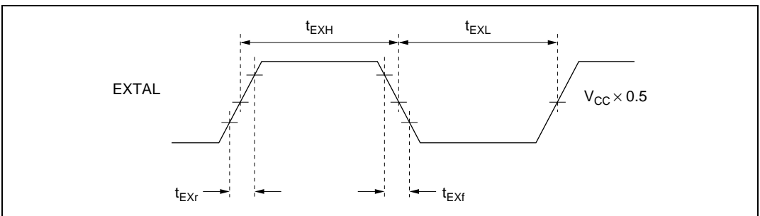
Figure 23A.7 External Clock Input Timing
