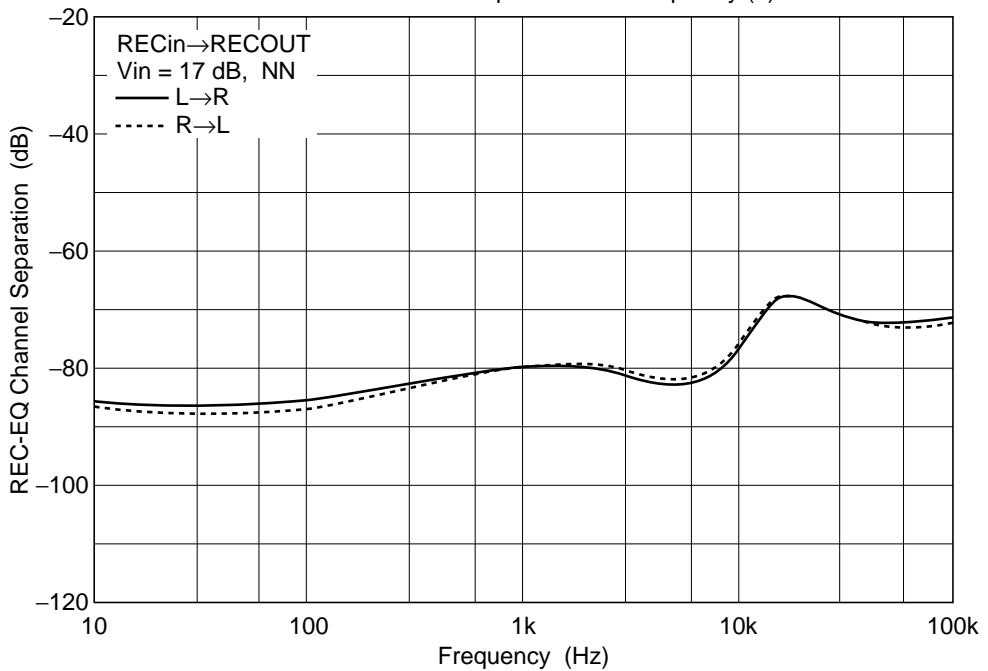
REC-EQ Channel Separation vs. Frequency (1)
