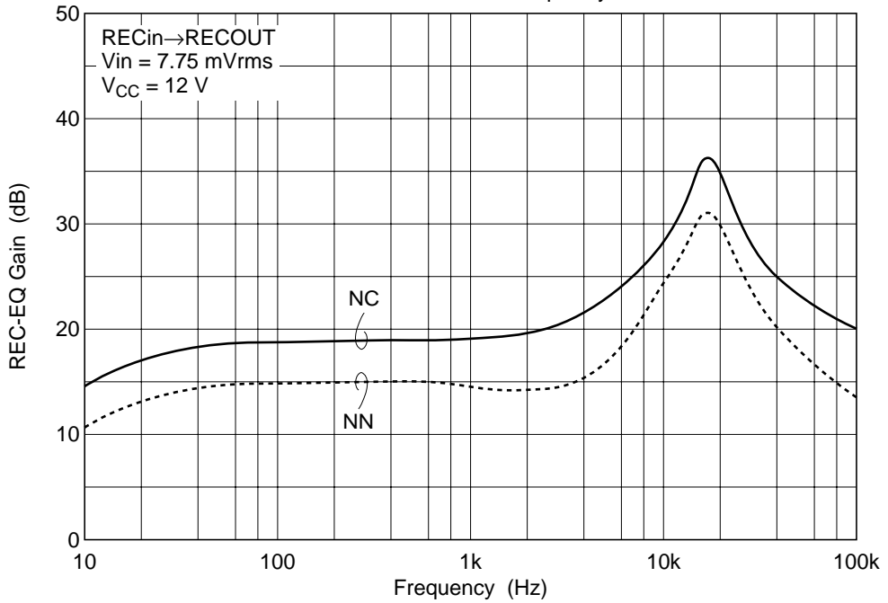
REC-EQ Gain vs. Frequency
