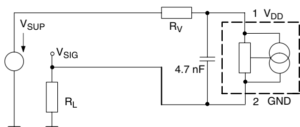
Fig. 5–2: Application Circuit 2
