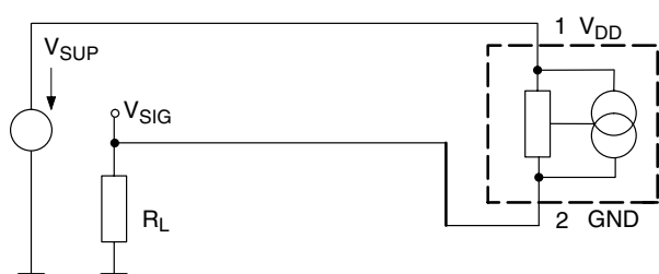
Fig. 5–1: Application Circuit 1
