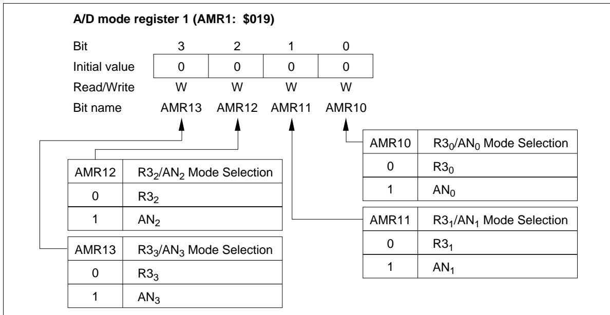
Figure 46 A/D Mode Register 1 (AMR1)
