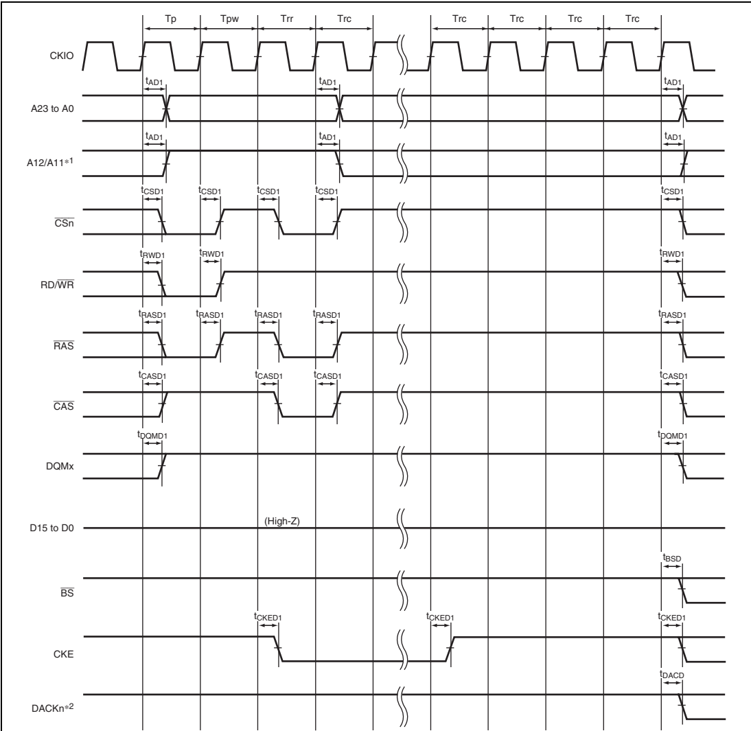
Figure 38.35 Self Refresh Timing of SDRAM (TRP = 2 Cycles)
