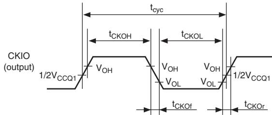
Figure 38.2 CKIO Clock Output Timing
