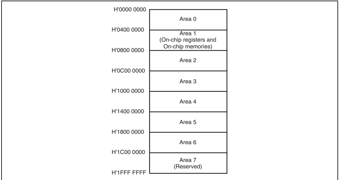
Figure 4.5 Physical Address Space
