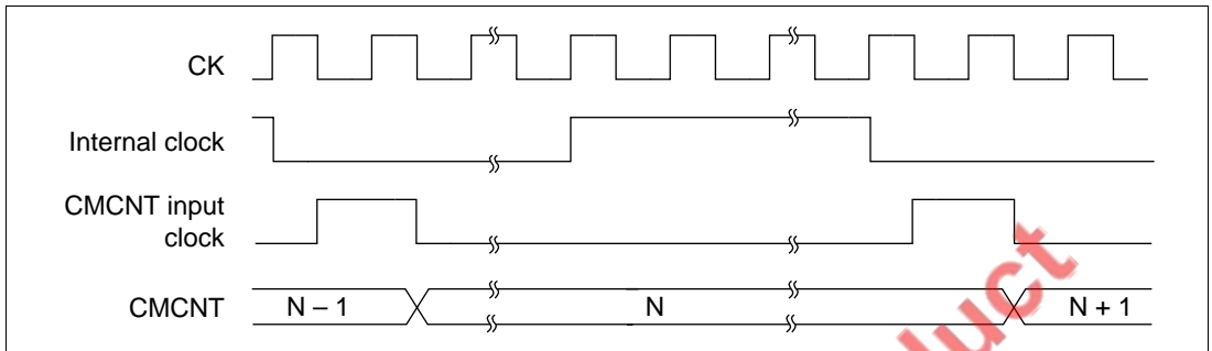
Figure 10.3 Count Timing
