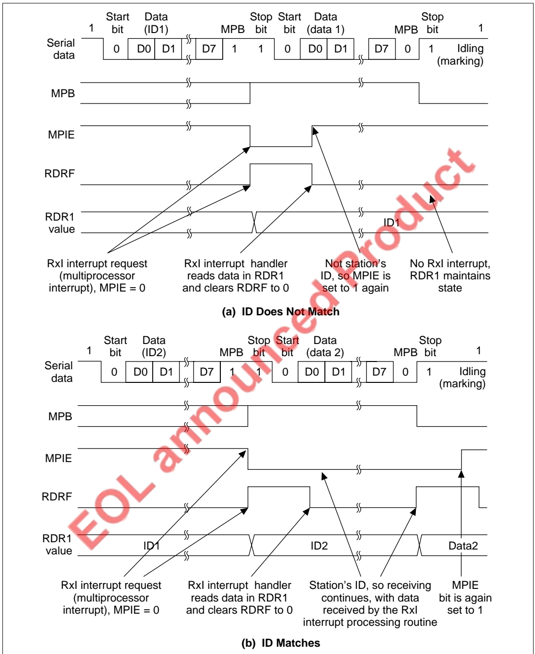
Figure 12.13 SCI1 Receive Operation (8-Bit Data with Multiprocessor Bit and One Stop Bit)
