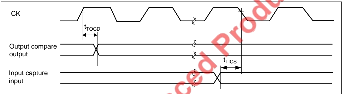
Figure 19.9 MTU Input/Output Timing
