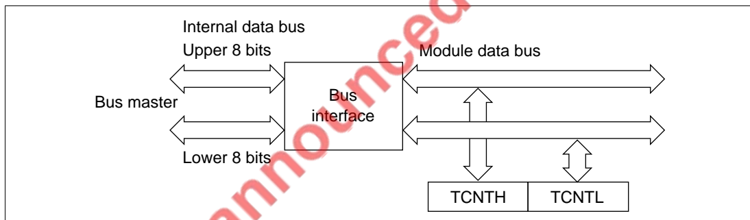
Figure 8.2 16-Bit Register Access Operation (Bus Master ↔ TCNT (16 Bits))
