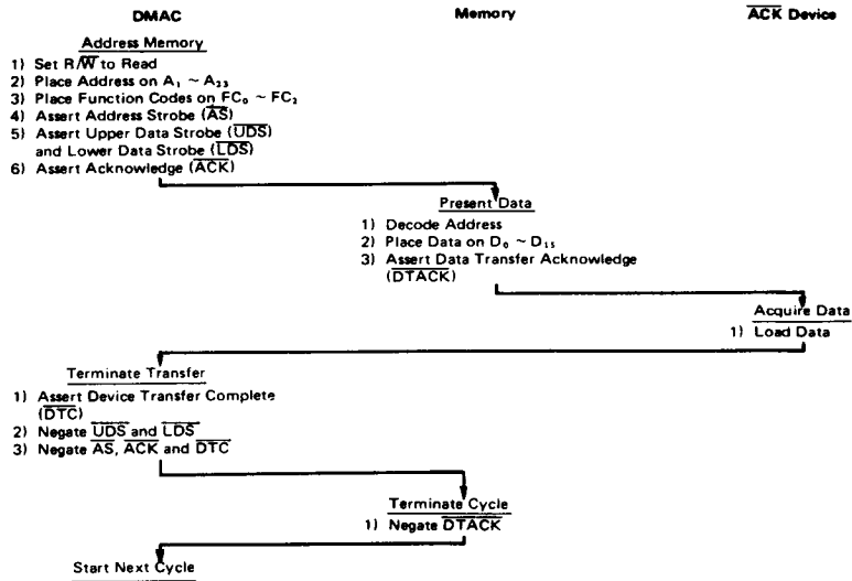
Figure 28 Word from Memory to Device with \overline{ACK}
