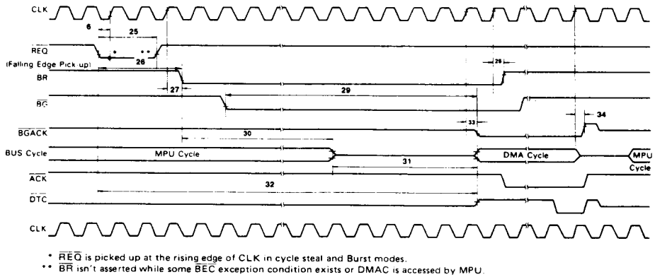
Figure 4 AC Electrical Waveforms – Bus Arbitration
