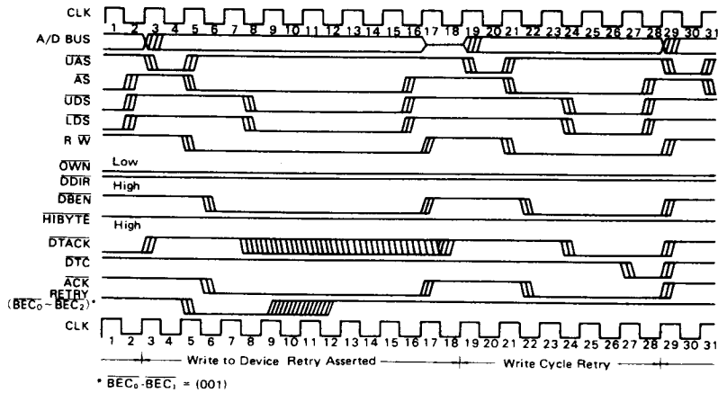
Figure 41 Retry Operation
