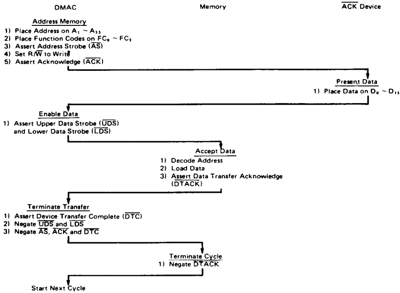
Figure 29 Word from Device with \overline{ACK} to Memory
