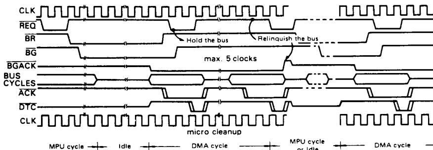
Figure 17 Cycle Steal Mode Request Timing
