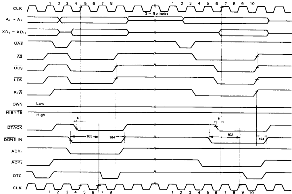
Figure 8 AC Electrical Waveforms – \overline{\text{DONE}} Input
