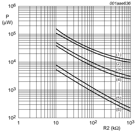
R1 = \infty ; VCO_IN at V_{SS} (0\text{ V}) ; C_L = 50\text{ pF} . Lines (1) and (2): V_{DD} = 15\text{ V} ; Lines (3) and (4): V_{DD} = 10\text{ V} ; Lines (5) and (6): V_{DD} = 5\text{ V} ; Lines (1), (3), and (5): C1 = 50\text{ pF} ; Lines (2), (4), and (6): C1 = 1\text{ }\mu\text{F} .
