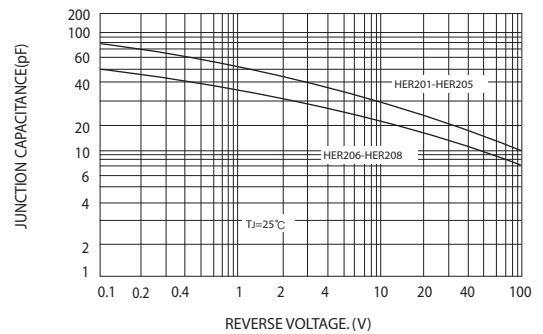
FIG.6-TYPICAL JUNCTION CAPACITANCE
