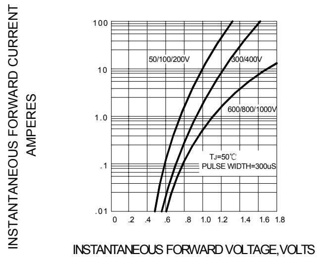
FIG.3–TYPICAL FORWARD CHARACTERISTICS
