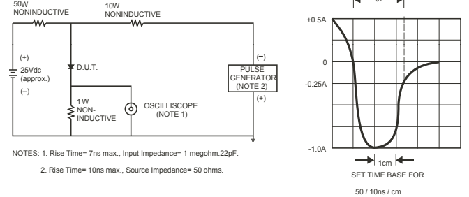
FIG. 6-Reverse Recovery Time Characteristic and Test Circuit
