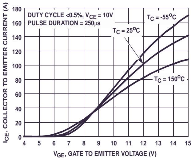
FIGURE 13. TRANSFER CHARACTERISTIC
