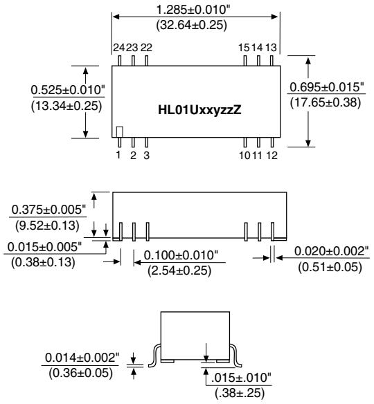
SMD PACKAGE
