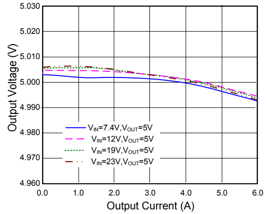
Load Regulation ( V_{BYP}=3.3V, MODE=High )
