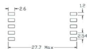
Recommended PCB Pattern
