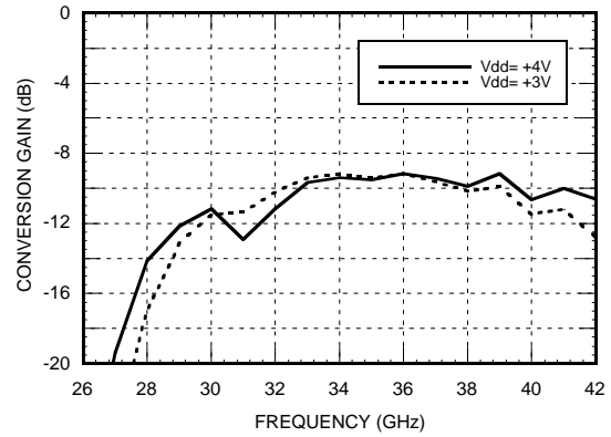
Conversion Gain, LO = +2 dBm, Vdd = +4V
