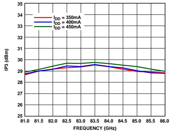
Figure 20. Output IP3 vs. Frequency at Various Drain Currents ( I_{DD} ), P_{OUT}/Tone = 12 dBm
