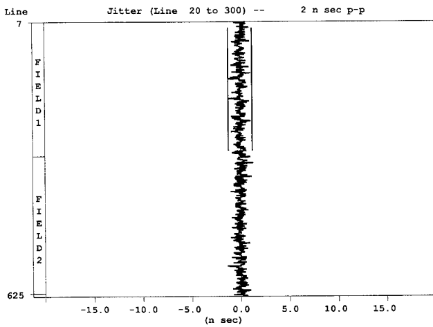
FIGURE 34. H SYNC JITTER IN A FRAME (PAL)
