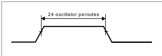
Figure 4-44 Reset Timing
