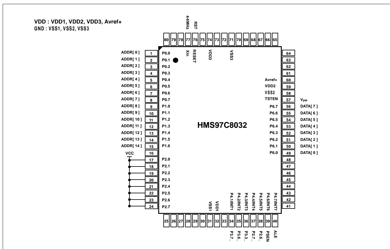
Figure 8-1 Pin Confiuration in OTP Diagram Mode
