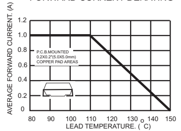
FIG.2- MAXIMUM AVERAGE FORWARD CURRENT DERATING
