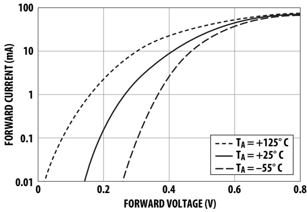
Figure 1. Typical Forward Current vs. Forward Voltage at Three Temperatures.
