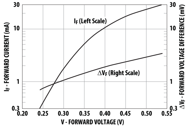
Figure 2. Typical VF Match, HSMS-820X Pairs and Quads.
