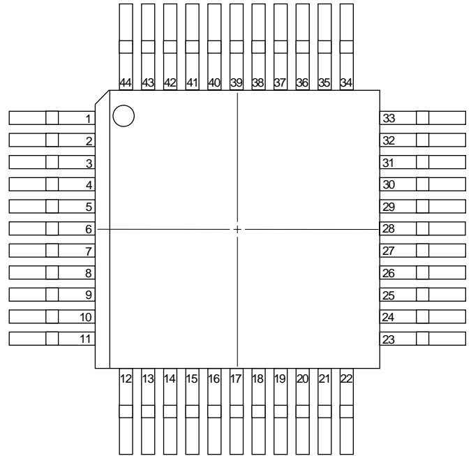
top view 44-pin Quad Plastic Gullwing Package
