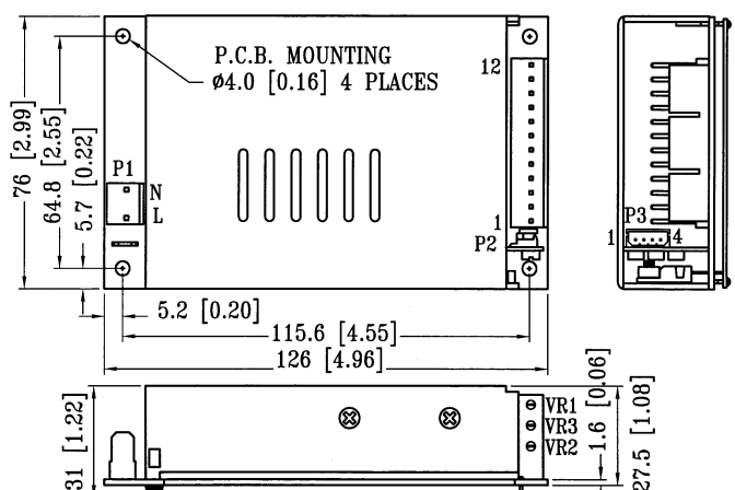
QUAD OUTPUT
