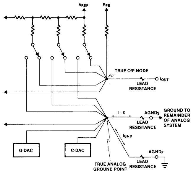
FIGURE 6. GROUND CONNECTIONS
