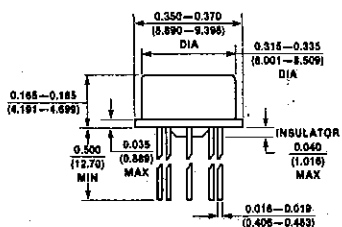
TO-78
