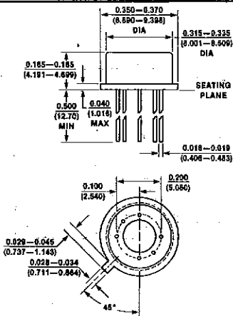
TO-78
