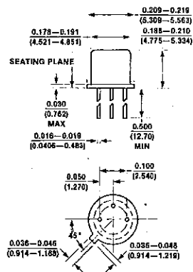
TO-18
