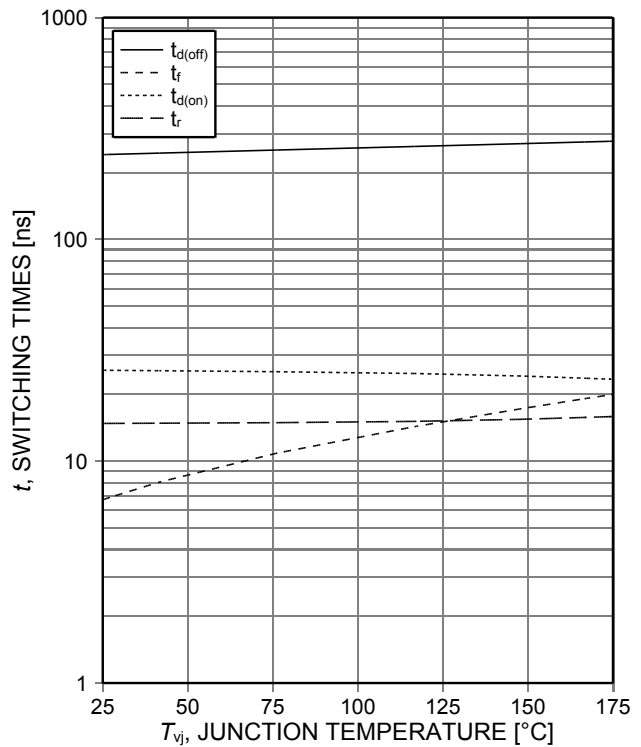
Figure 10. Typical switching times as a function of junction temperature (inductive load, V_{CE}=400\text{V} , V_{GE}=15/0\text{V} , I_C=20\text{A} , r_G=23\Omega , Dynamic test circuit in Figure E)
