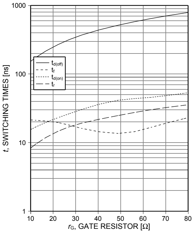
Figure 9. Typical switching times as a function of gate resistor (inductive load, T_{vj}=175^{\circ}\text{C} , V_{CE}=400\text{V} , V_{GE}=15/0\text{V} , I_C=20\text{A} , Dynamic test circuit in Figure E)
