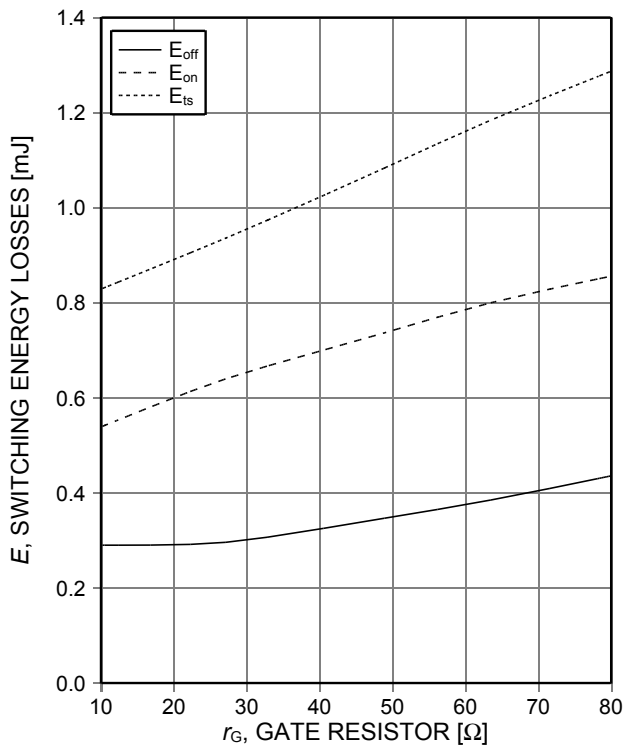
Figure 13. Typical switching energy losses as a function of gate resistor (inductive load, T_{vj}=175^{\circ}\text{C} , V_{CE}=400\text{V} , V_{GE}=15/0\text{V} , I_C=20\text{A} , Dynamic test circuit in Figure E)
