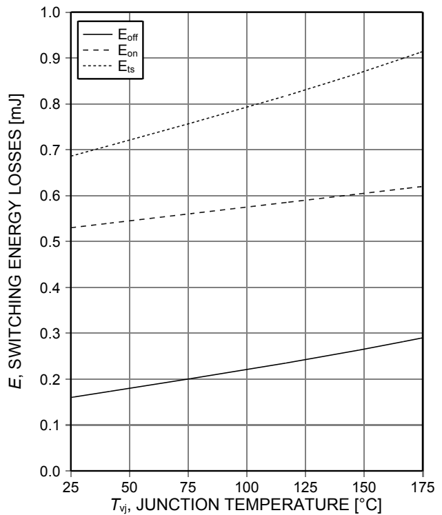
Figure 14. Typical switching energy losses as a function of junction temperature (inductive load, V_{CE}=400\text{V} , V_{GE}=15/0\text{V} , I_C=20\text{A} , r_G=23\Omega , Dynamic test circuit in Figure E)
