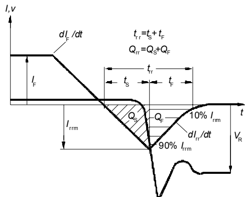
Figure B. Definition of diodes switching characteristics
