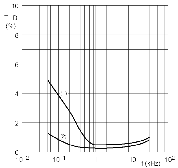
Figure 8. Total harmonic distortion versus frequency.
