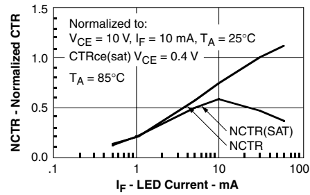
Figure 5. Normalized non-saturated and saturated CTR at T A =85°C versus LED current
