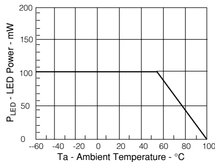
Figure 6. Maximum LED power dissipation
