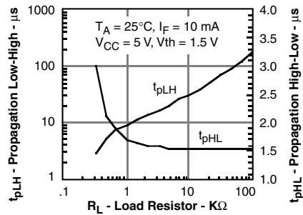
Figure 17. -1 Propagation delay versus collector load resistor
