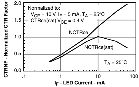
Figure 12. Normalization factor for non-saturated and saturated CTR TA=50°C versus IF
