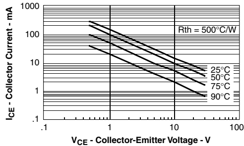
Figure 10. Maximum collector current versus collector voltage
