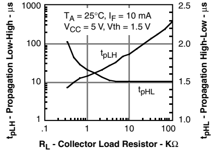
Figure 19. -4 Propagation delay versus collector load resistor
