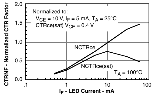
Figure 14. Normalization factor for non-saturated and saturated CTR TA=85°C versus IF
