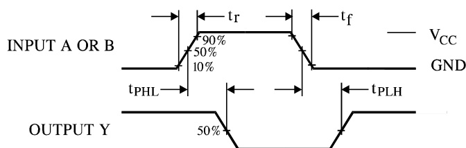
Figure 1. Switching Waveforms
