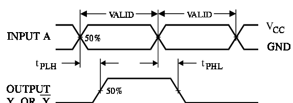
Figure 2. Switching Waveforms
