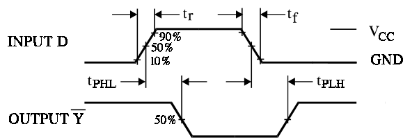
Figure 3. Switching Waveforms
