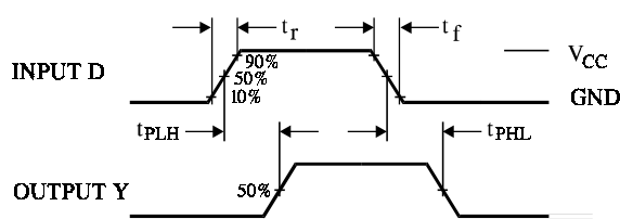
Figure 1. Switching Waveforms
