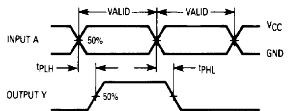
Figure 2. Switching Waveforms
