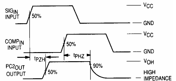
Figure 2. Switching Waveforms
