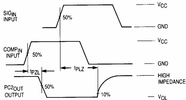
Figure 3. Switching Waveforms
