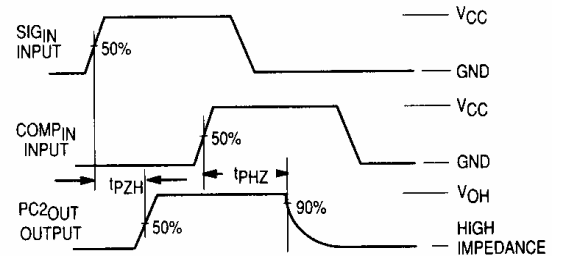
Figure 2. Switching Waveforms
