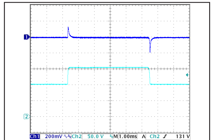
Figure 6: Output voltage response to step-change in input voltage (1000 V/ms). Load cap: 100 µF, electrolytic output capacitance. Ch 1: V out (200 mV/div), Ch 2: V in (50 V/div).
