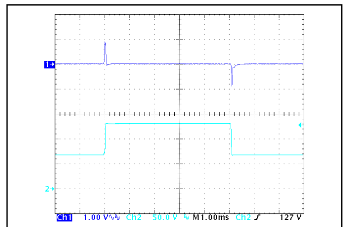
Figure 6: Output voltage response to step-change in input voltage (500 V/ms). Load cap: 100 µF, electrolytic output capacitance. Ch 1: V out (1 V/div), Ch 2: V in (50 V/div).
