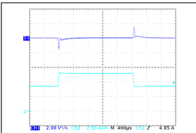
Figure 5: Output voltage response to step-change in load current (50%-75%-50% of Iout(max); dl/dt = 0.1 A/us). Load cap: 1 μF ceramic capacitor. Ch 1: Vout (2 V/div), Ch 2: Iout (2.5 A/div).
