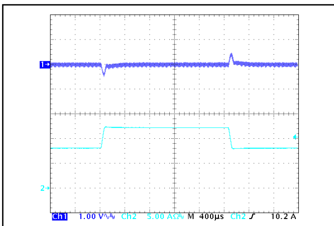
Figure 5: Output voltage response to step-change in load current (50%-75%-50% of I out (max)); dI/dt = 0.1 A/µs. Load cap: 15 µF Tantalum + 1 µF Ceramic capacitor. Ch 1: V out (1 V/div), Ch 2: I out (5 A/div).
