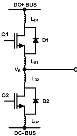
Figure 10: Parasitic Elements
