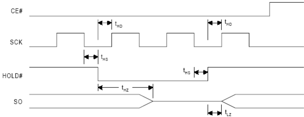
Figure 32. HOLD TIMING
