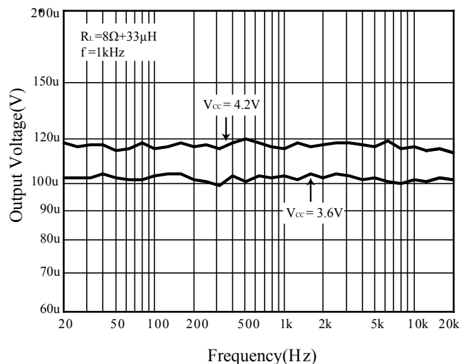
Figure 20 Noise
