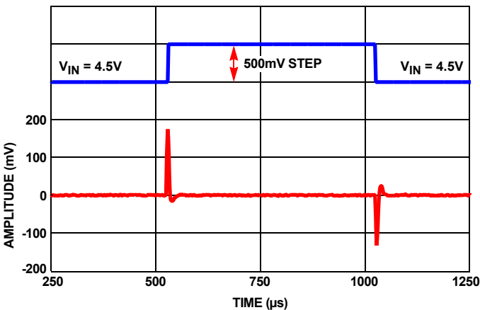
FIGURE 40. LINE TRANSIENT WITH 0.1\mu F LOAD
