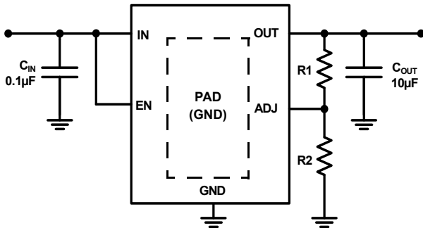
FIGURE 1. TYPICAL APPLICATION
