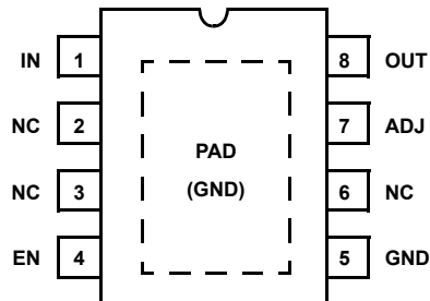
ISL80136 (8 LD EPSON) TOP VIEW
