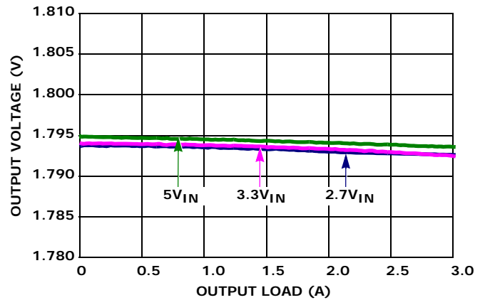
FIGURE 34. V_{OUT} REGULATION vs LOAD, 1.8V_{IN} DUAL CHANNEL 1, T_A = +25^\circ C
