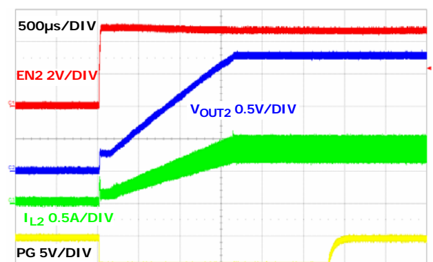
FIGURE 29. SOFT-START AT FULL LOAD CHANNEL 2
