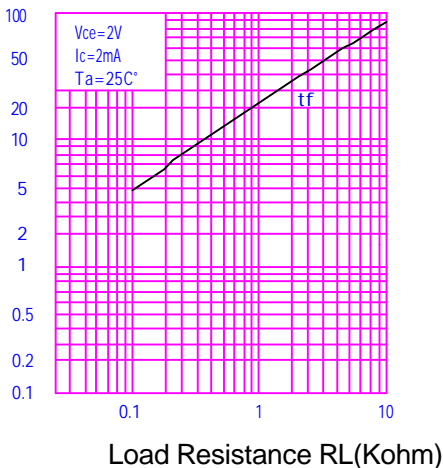
Fig.11 Response Time vs. Load Resistance
