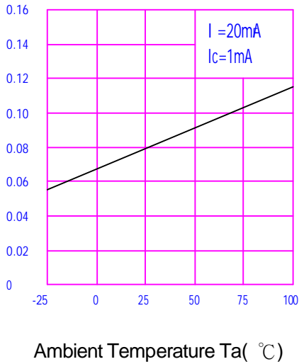
Fig.8 Collector-emitter Saturation Voltage vs. Ambient Temperature
